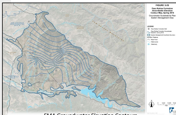
EMA Groundwater Elevation Contours
