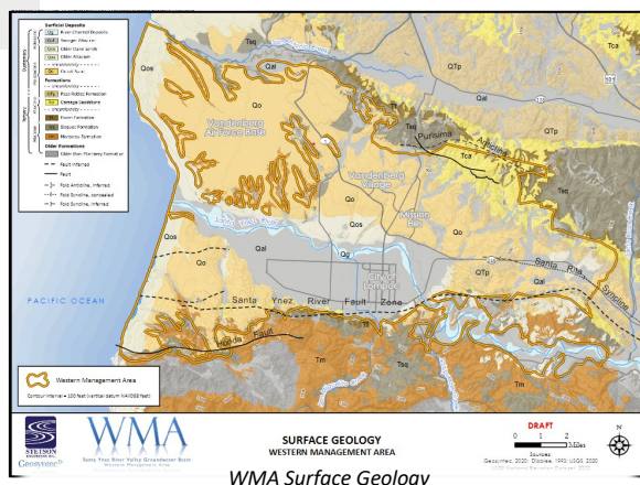
WMA Surface Geology
